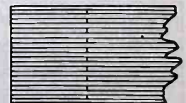
The Upper Sketches Show the Path of the Eddy Currents in a Plain Iron Core and How They Are Suppressed When Laminations Are Used. The Lower Ones Give the Method of Interleaving the Sheets Composing the Core.
