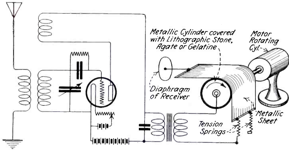
This diagram shows the loud talker illustrated on the front cover of this magazine, connected to a radio receiver. The functioning of this instrument may be understood by referring to the sketch.
