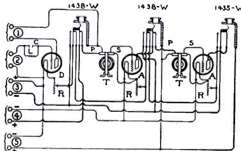
DETECTOR & 2 STAGE AMPLIFIER USING FILAMENT CONTROL JACKS
