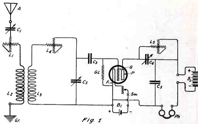
Fig. 1 Complete Hook-up of the Set With Indications of the Various Parts.
