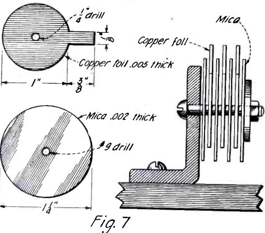
Fig. 6 Shows the Connections of the Coils in the Variometer. In Fig. 7 Are the Details of Construction of the Small Fixed Condenser.
